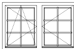
26 ISO 70 mm 1530 x 990 mm 2x
